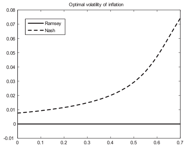
Fig. 5. Optimal inflation volatility under Ramsey and under Nash
